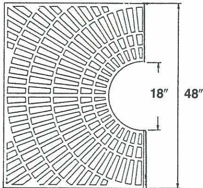
Half Section
